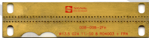
2" Grounded Coplanar Waveguide (GCPWG) on 8 mil RO4003 with FR-4 Backer
