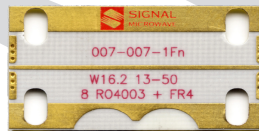
1" Microstrip on 8 mil RO4003 with FR-4
