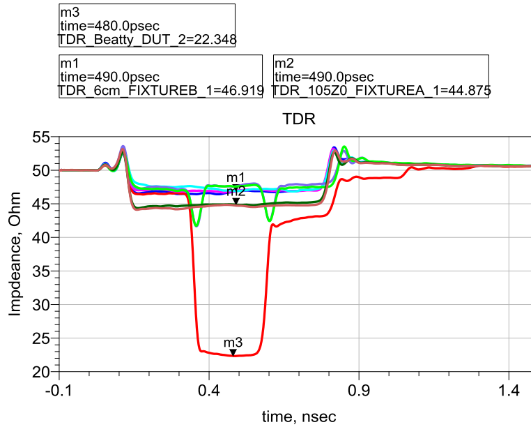
Figure 4. Impedance profiles for test coupons
