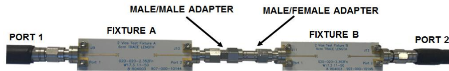
Figure 5: Setup example picture for measuring the 2x-thru of the test fixture.
