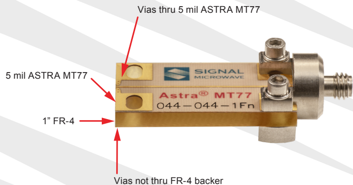
1" Microstrip on 5 mil ISOLA ASTRA MT77 with FR-4 Backer
